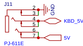
Lisa Keyboard Port
