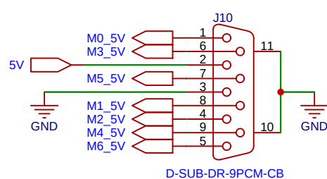
Lisa Mouse Port
