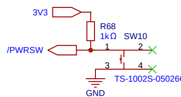
Soft Power Button
